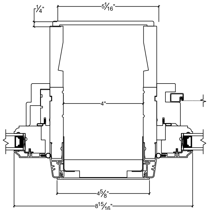
Transom & Casement Clad Mull 3 1/2" Jamb c/w 4" Pocket
