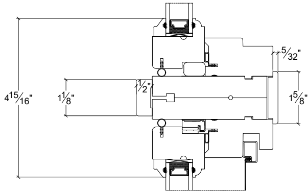
TRANSOM / CASEMENT STACK
