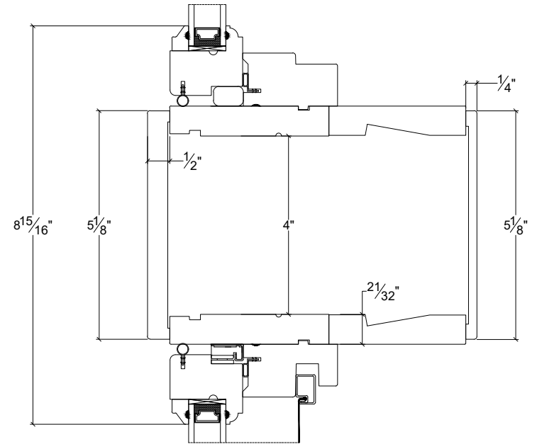
TRANSOM / CASEMENT STACK
