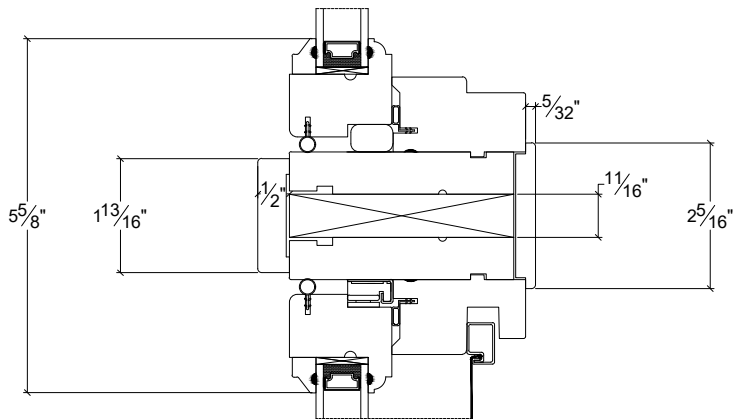
TRANSOM / CASEMENT STACK
