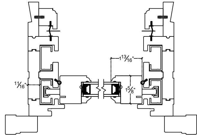
Top Sash
