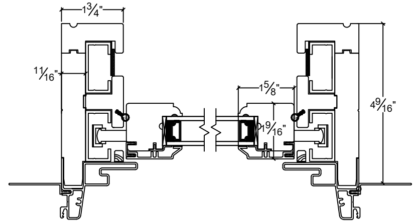
Top Sash
