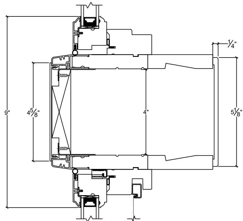
TRANSOM / CASEMENT CLAD STACK
