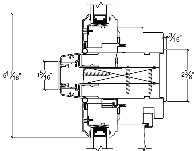
TRANSOM / CASEMENT CLAD STACK
