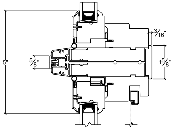
TRANSOM / CASEMENT CLAD STACK
