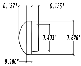
WOOD PLUG
