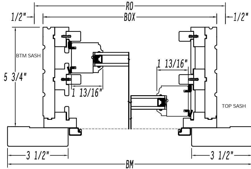
Horizontal Cross-section
