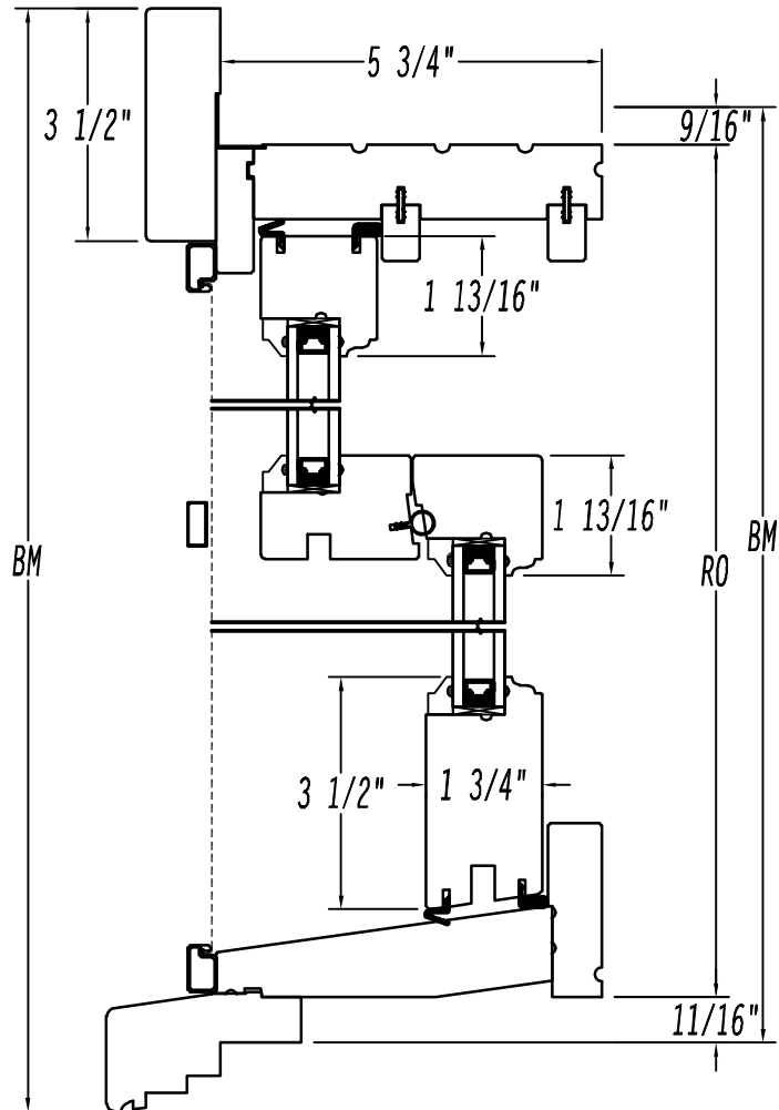
Vertical Cross-section
