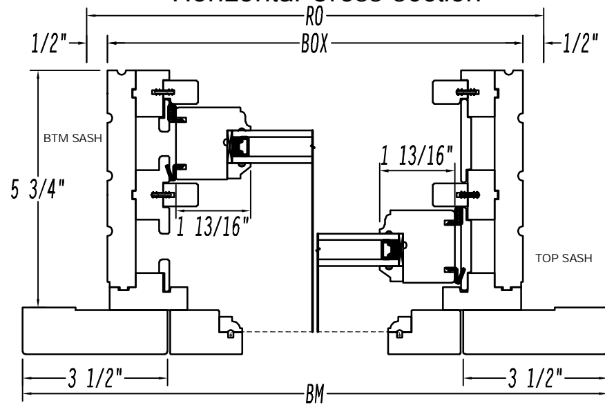
Horizontal Cross-section
