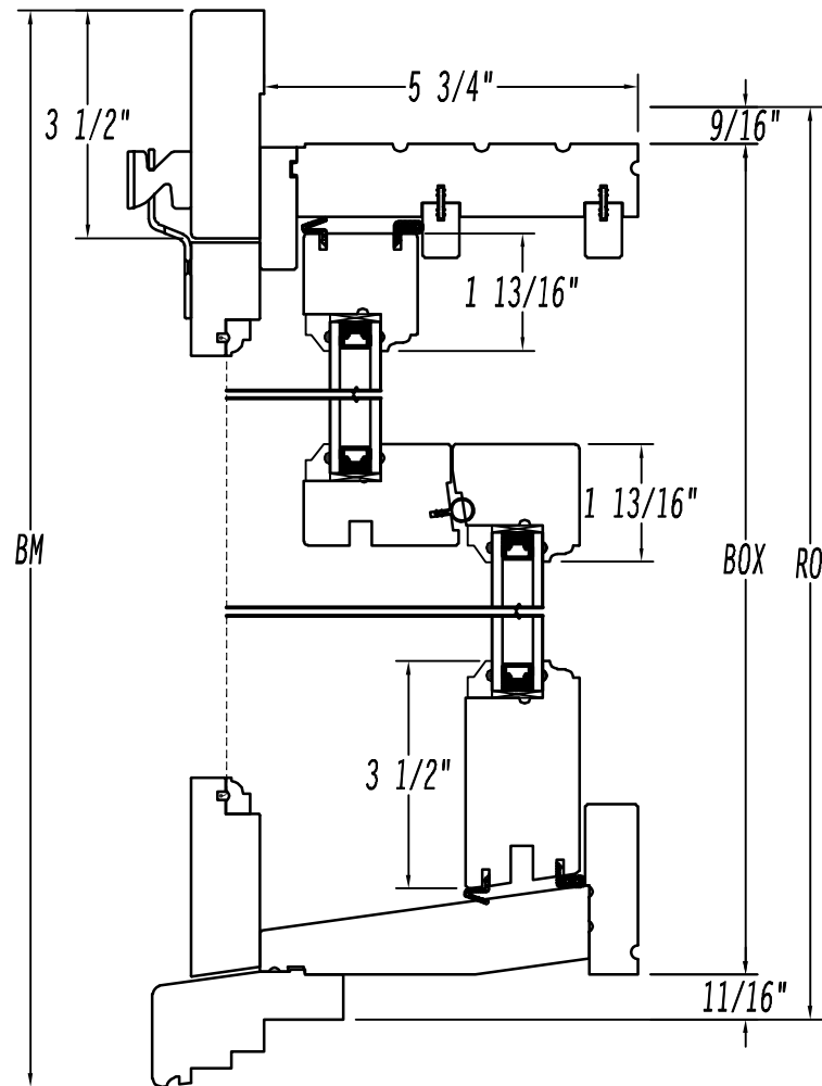
Vertical Cross-section
